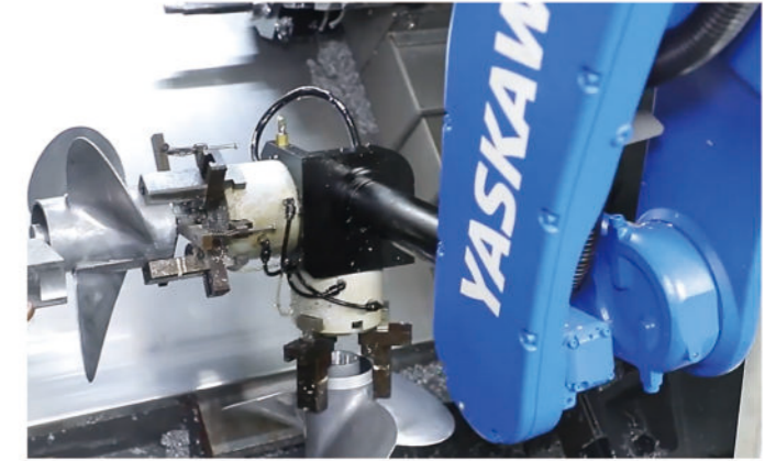
Advanced 6-axis linkage robotic arm
